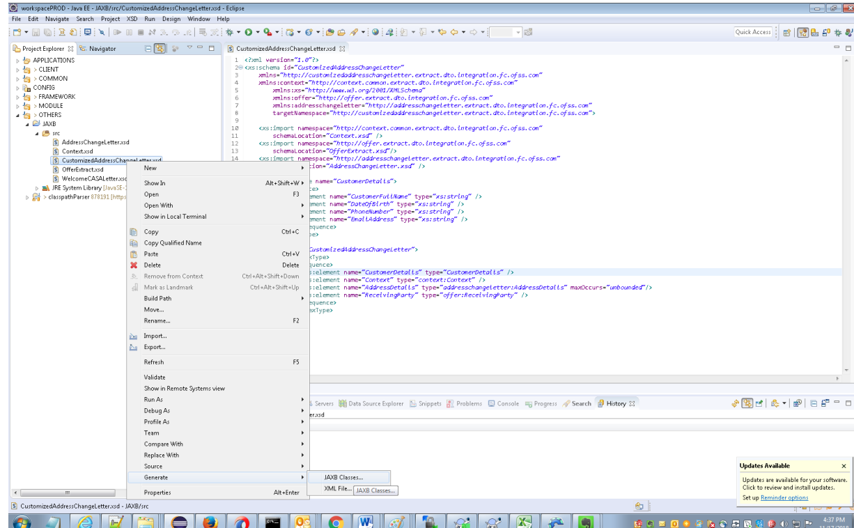
Figure 19–9 Generate JAXB Classes from Customized XSD
