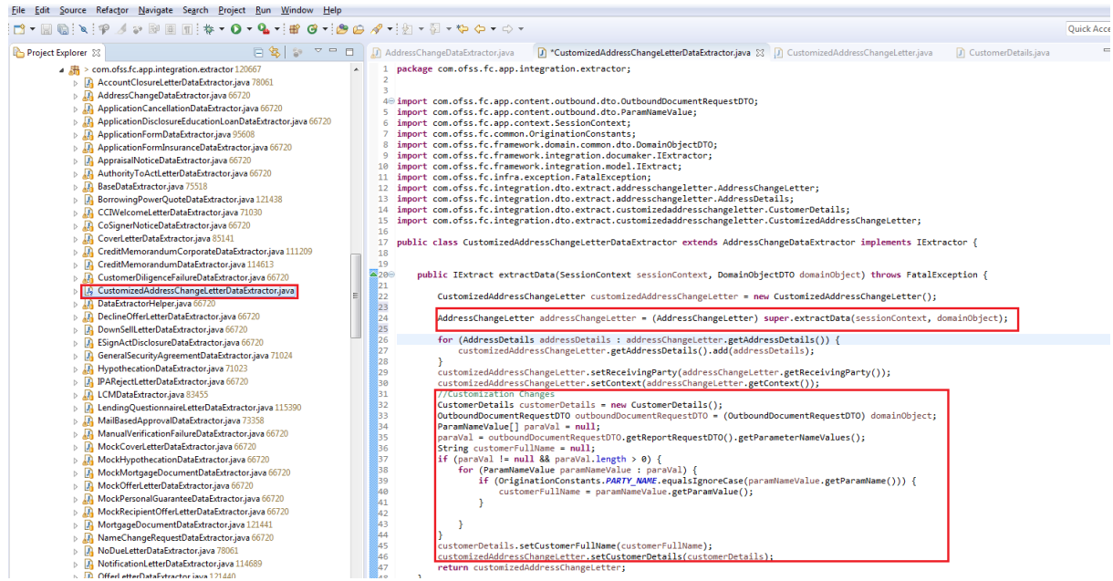
Figure 19–13 Customized AddressChangeLetterDataExtractor
